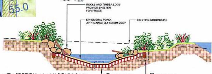
SECTION AA - HABITAT POND 1:50
