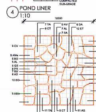
MATRIX B (324m2) - PLANT SCHEDULE
