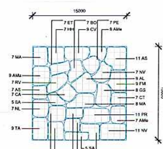
MATRIX C (225m2) - PLANT SCHEDULE
