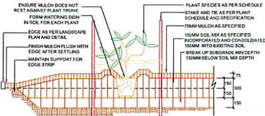
1 MASS PLANTING 1:20
