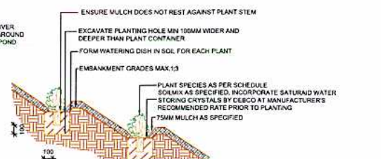
2 TUBESTOCK PLANTING 1:20
